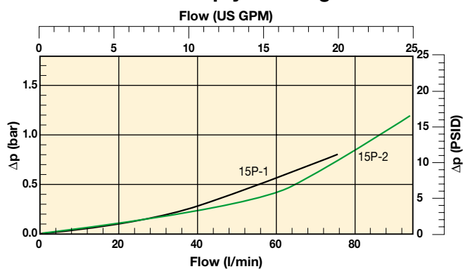
15P Empty Housing
